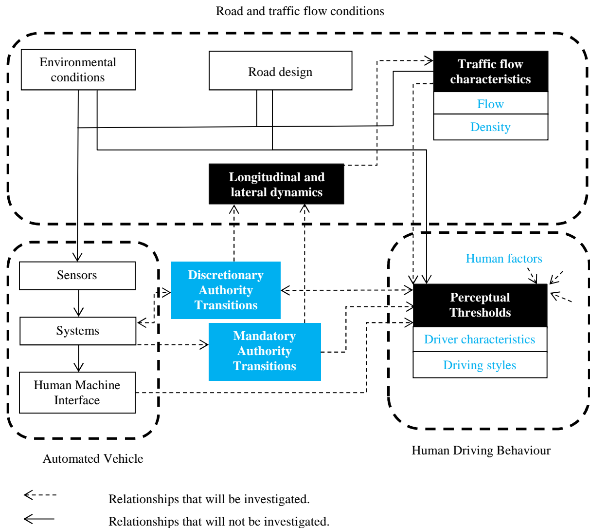
Figure 1 Theoretical framework of relationships between authority transitions, human factors and traffic flow conditions.
