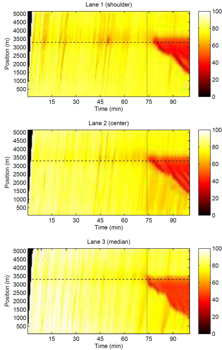
Figure 2. Speed contour plots (the color indicates the speed (km/h), the black dotted lines show the time at which traffic breaks down on the median lane, and the black dashed lines indicate the location at which the transition section ends)
