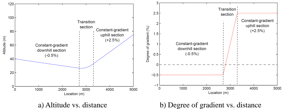
Figure 1. Representation of sag by means of three sections (Yamato sag, Tomei Expressway)
