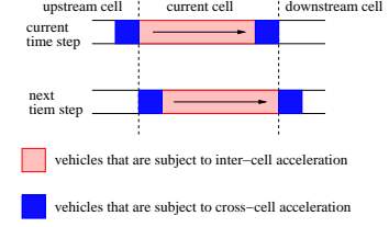
Fig. 2. Inter-cell acceleration and cross-cell acceleration
