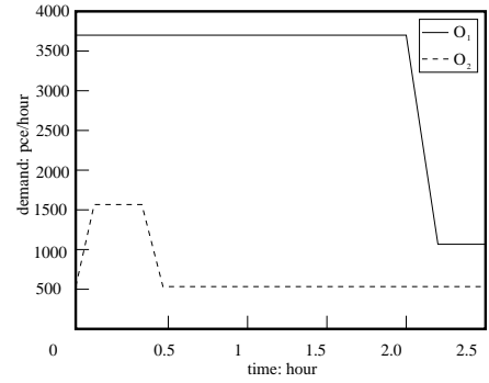
Fig. 5. The original demand scenario
